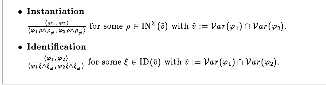
Figure 1: Derivation rules
