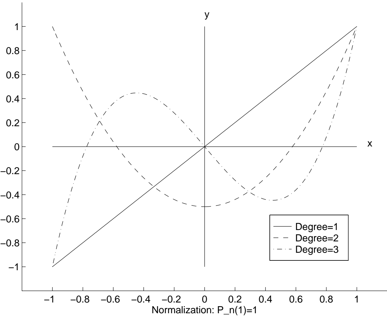
Legendre polynomials of degrees 1,2,3
