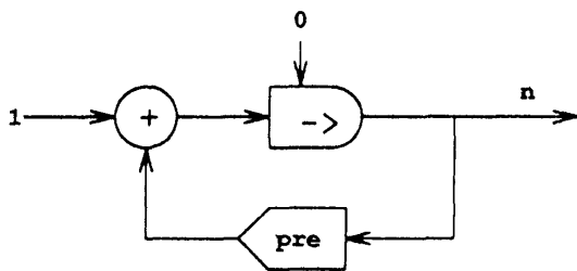
Fig. 2. Counter network.
