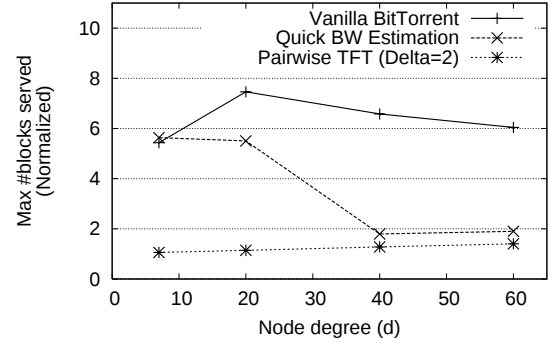
Figure 11: Maximum number of blocks (normalized by file size) served by any node during an experiment for (a) vanilla BitTorrent, (b) BitTorrent with QBE, and (c) with the pairwise block-level TFT policy.
