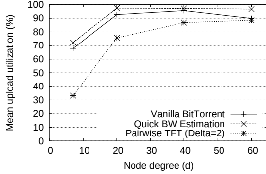
Figure 10: Mean upload utilization for (a) vanilla BitTorrent, (b) BitTorrent with QBE, and (c) with the pairwise block-level TFT policy.
