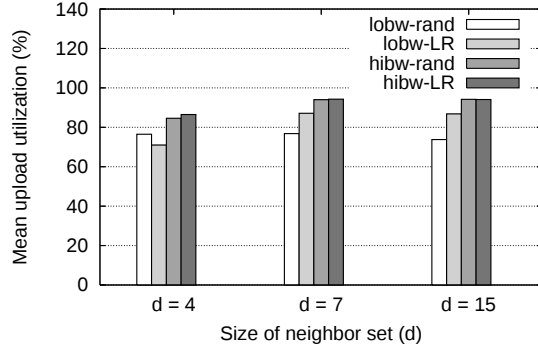
Figure 6: Upload utilization for LRF and Random policies for different values of the node degree, d . LRF performs better only when the node degree is large and the seed bandwidth is low.
