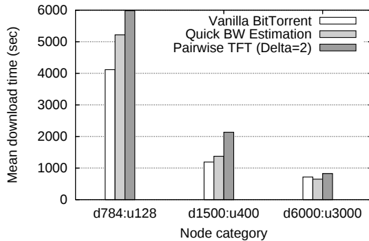
Figure 14: Download times for nodes of different categories for various schemes.
