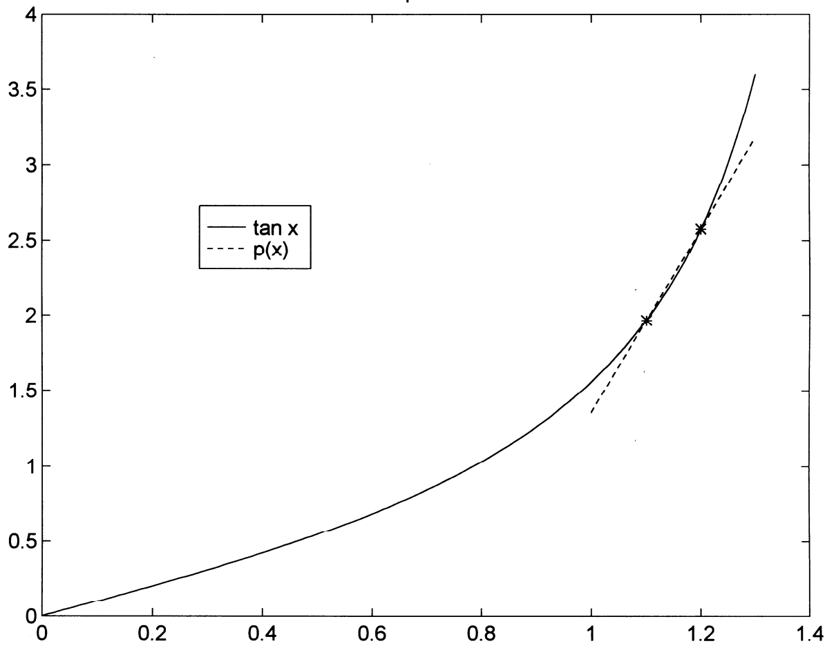
Linear interpolation of tan x
